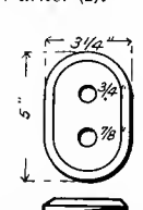
Figs. 1957-1958. Bevel Washer (4)
